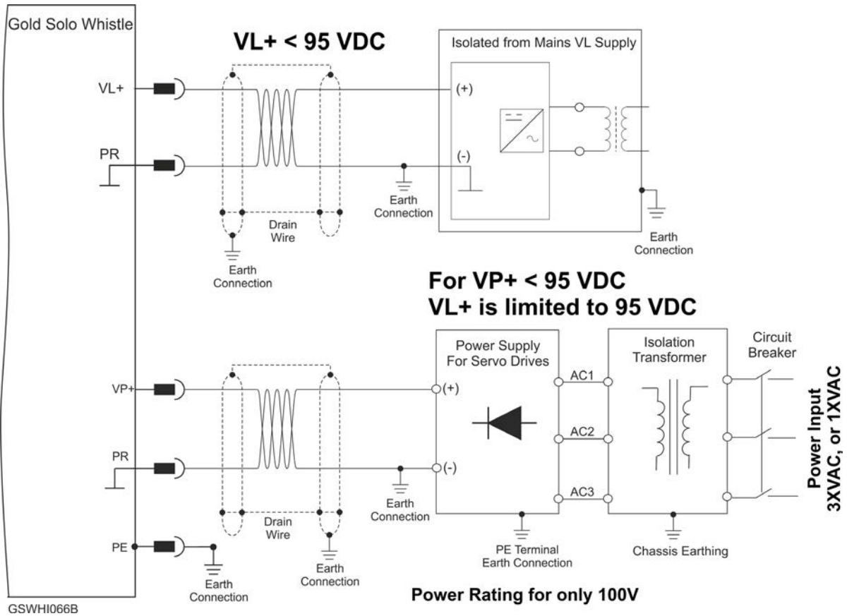
Figure 16: Control Supply Connection Diagram
