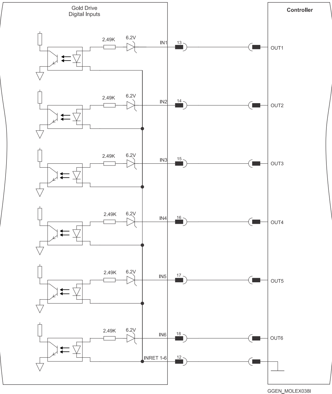
Figure 32: Digital Input Connection Diagram – Source PLC Option
