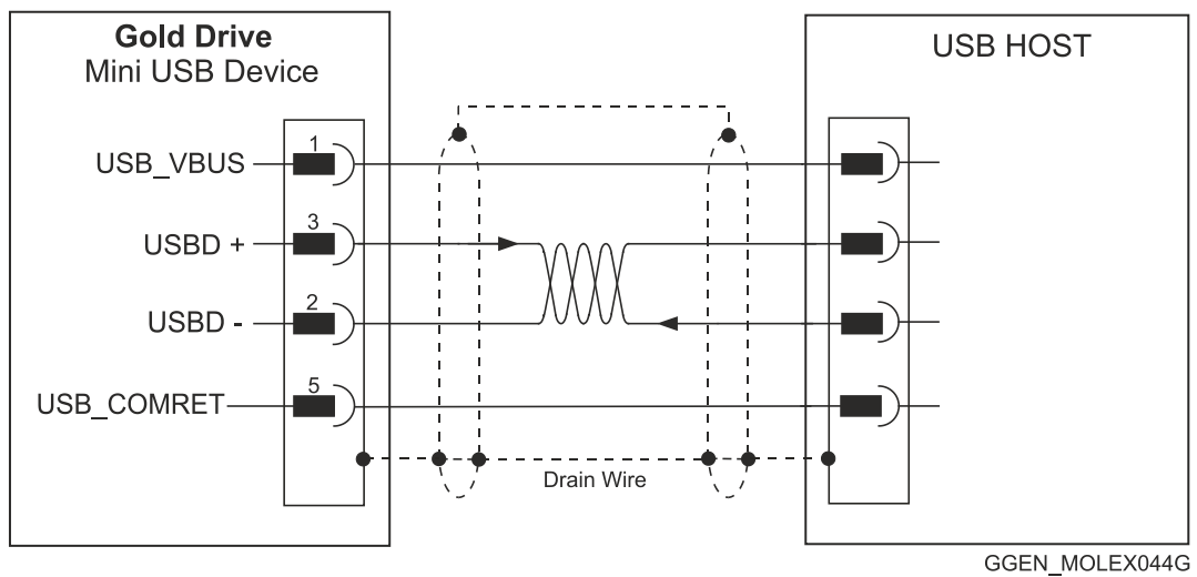
Figure 34: USB Network Diagram
