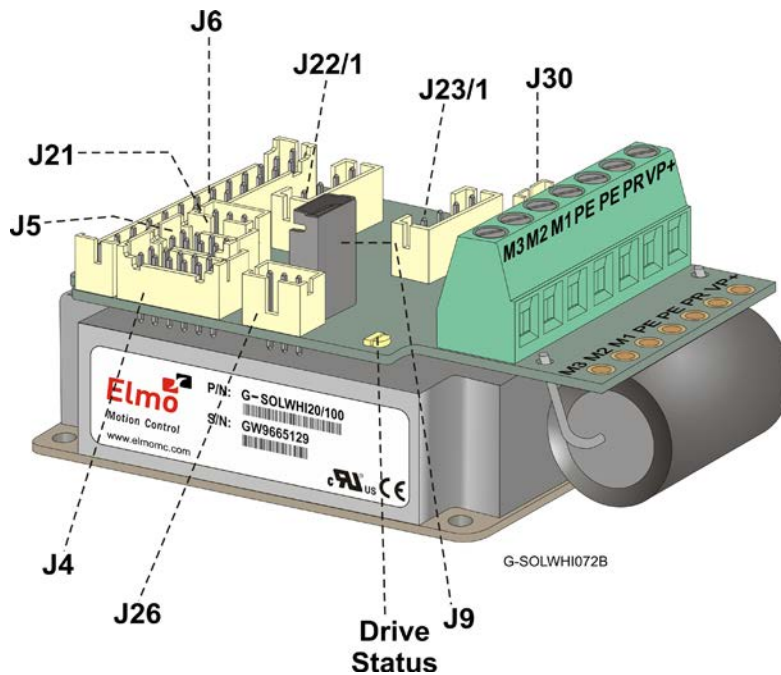
Figure 2: Connector Locations – CAN
