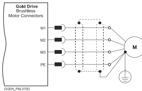
Figure 12: Brushless Motor Power Connection Diagram
