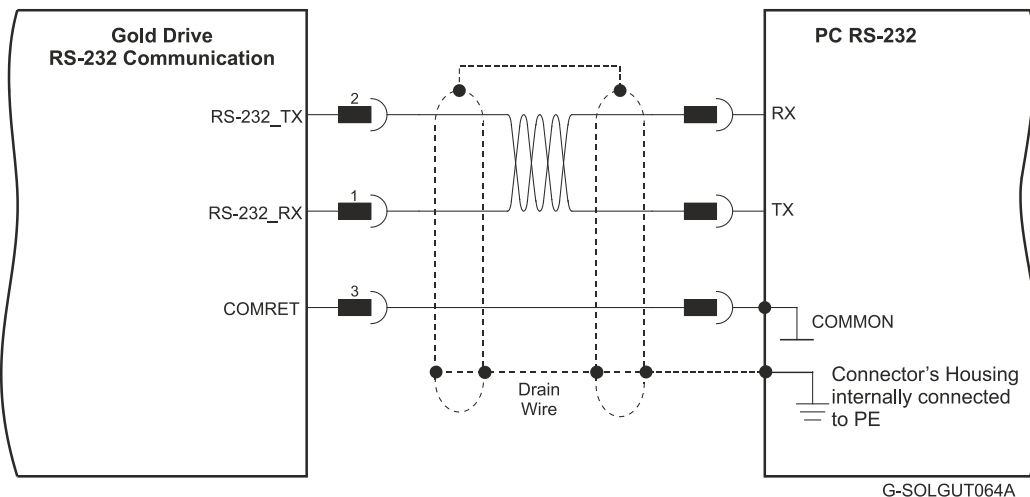
Figure 35: RS-232 Connection Diagram
