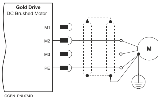
Figure 13: Brushed Motor Power Connection Diagram
