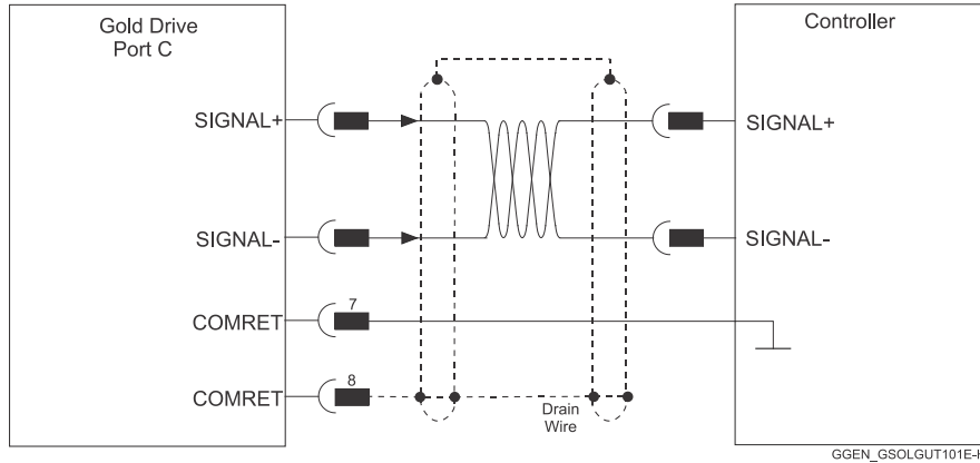
Figure 9: Feedback Port C Cable Assemblies
