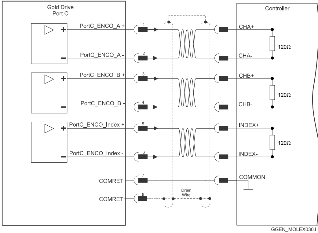
Figure 28: Emulated Encoder Differential Output – Recommended Connection Diagram
