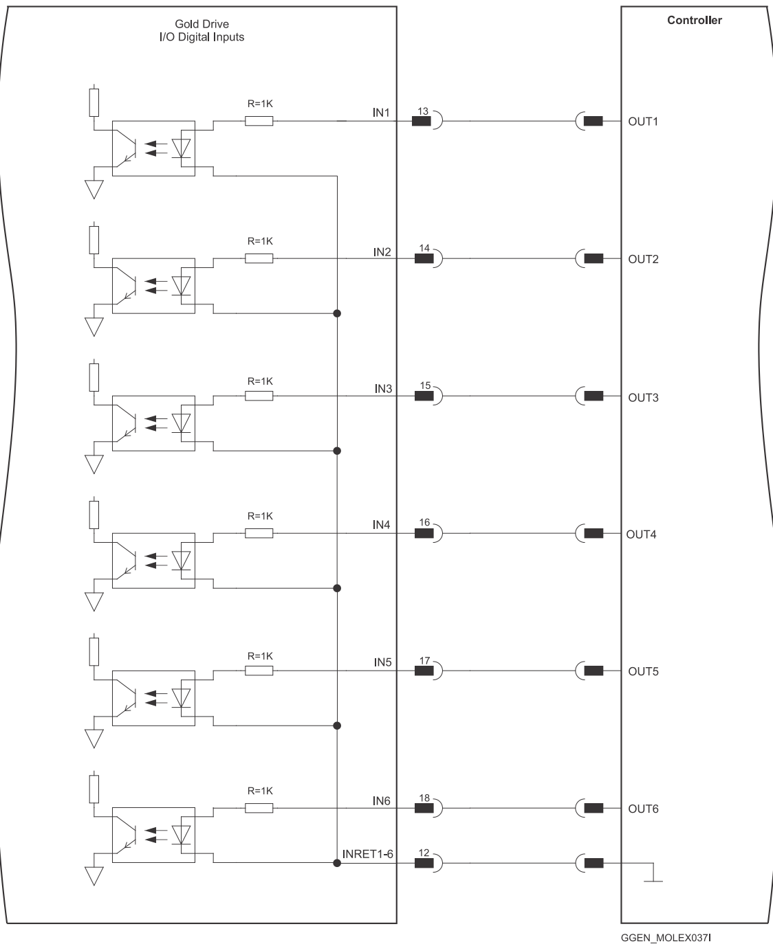
Figure 30: Digital Input TTL Mode Connection Diagram
