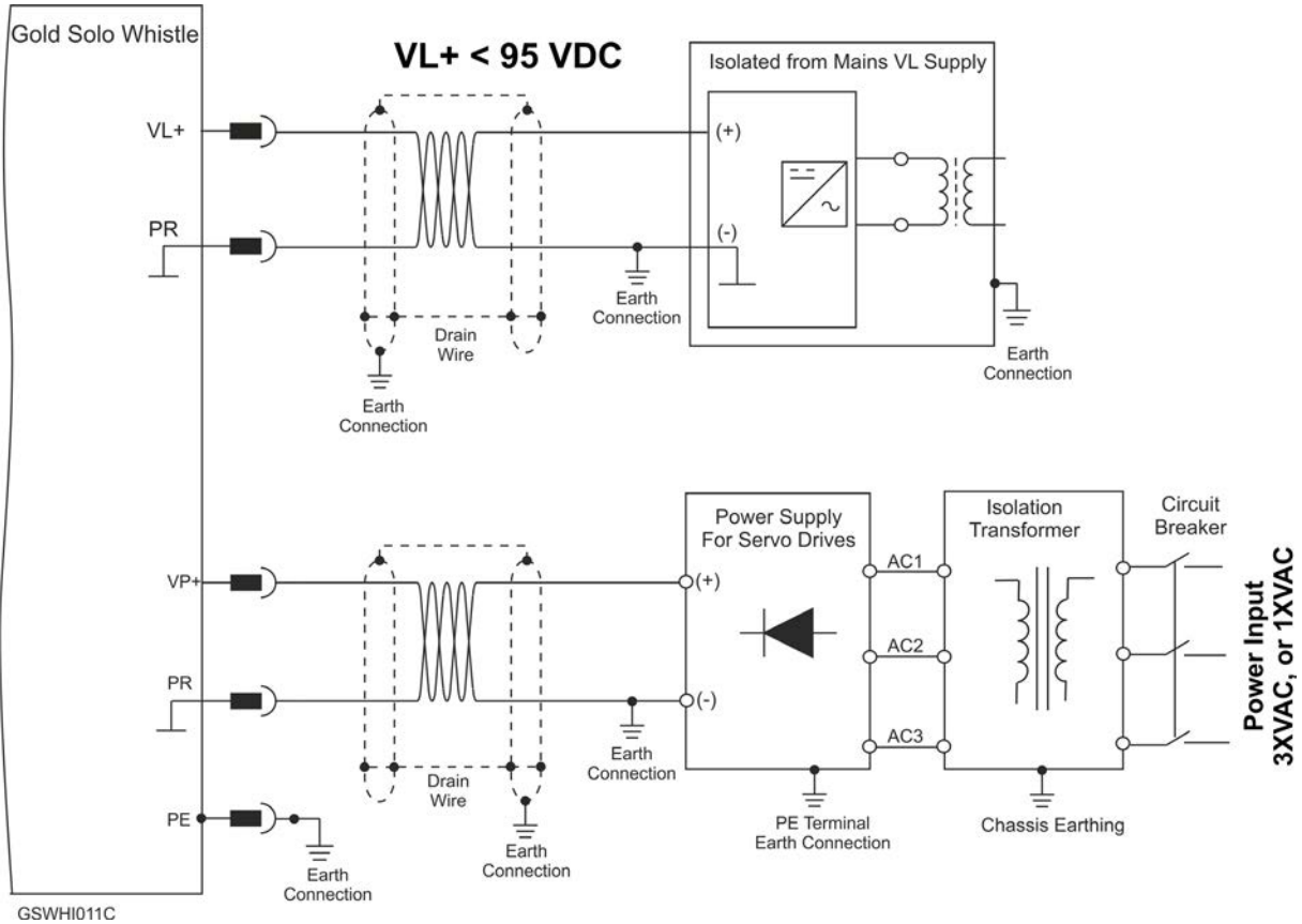
Figure 14: 200 VDC Power Source Connection Diagram
