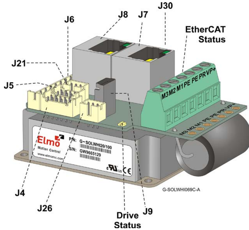
Figure 1: Connector Locations – EtherCAT
