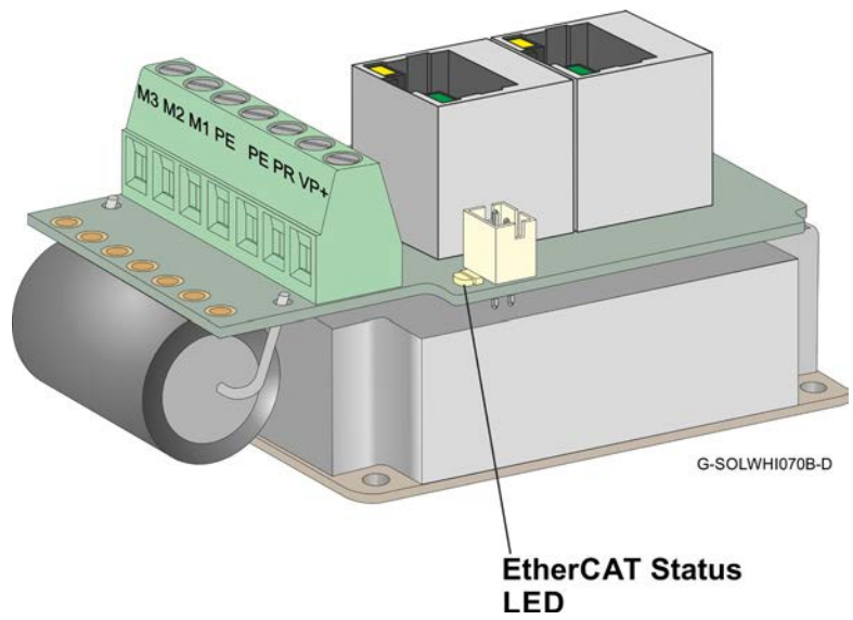
Figure 37: EtherCAT Status LED
