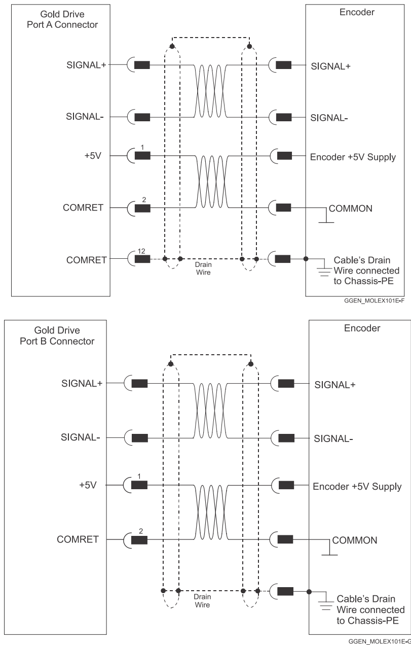
Figure 8: Feedback Port A and B Cable Assemblies
