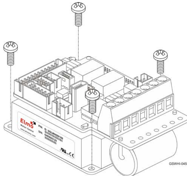
Figure 3: Mounting the Gold Solo Whistle
