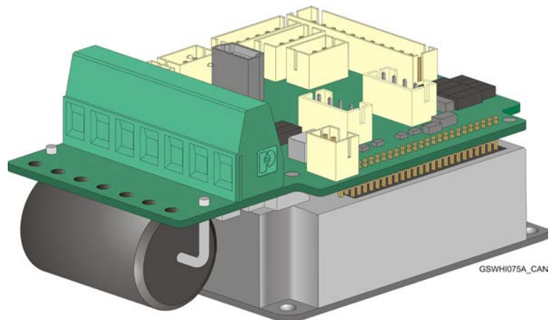
Figure 38: Gold Solo Whistle Status Indicator - CAN
